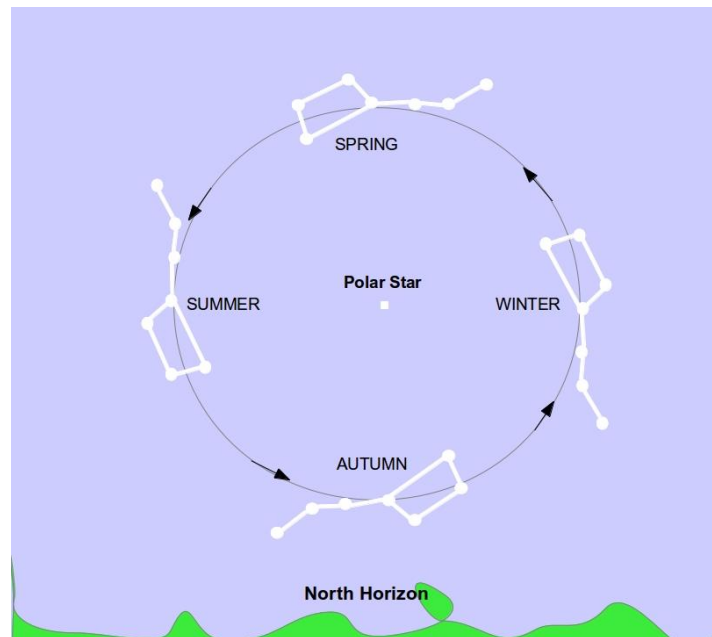
Fig. 10: Relative positions of the Ursa Major around the North Pole throughout the year (at the same hour).
