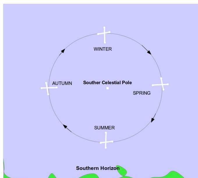
Fig. 11: Relative positions of the Southern Cross around the South Pole during the year (at the same hour).
