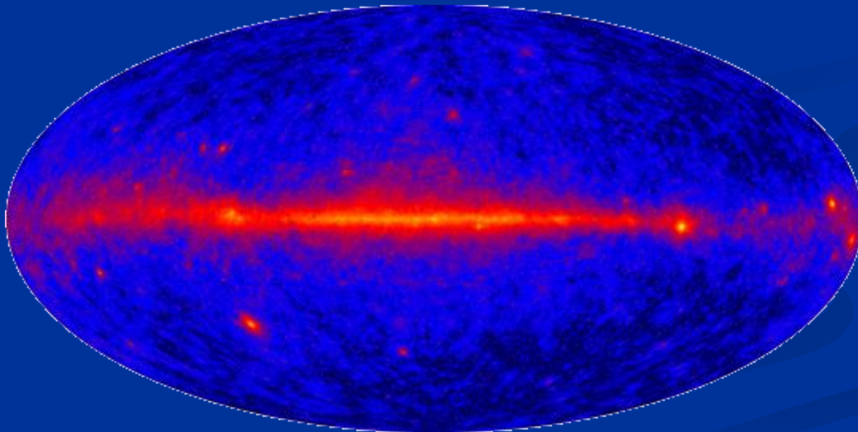
Fermi's Five-year View of the Gamma-ray Sky 费米伽玛巡天五年数据结果
