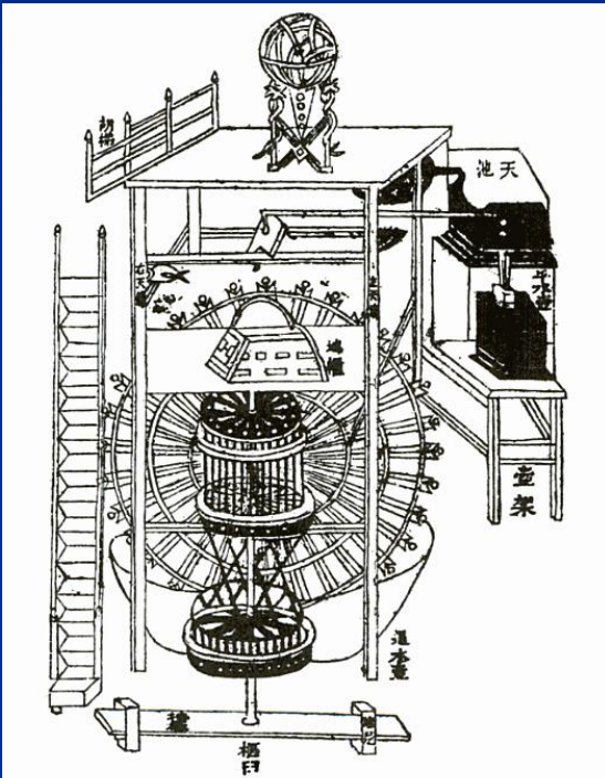
Fig. 651. General diagram of the works ( Hsin I Huang Fa Yao , ch. 3, p. 4a). On the right, the upper reservoir tank ( thien chih ) with the constant-level tank ( phing shui hu ) beneath it. In the centre, foreground, the 'earth horizon' box ( ti hui ) in which the celestial globe is mounted; below, the time-keeping shaft and wheels supported in the mortar-shaped end-bearing ( shu chiu ). Behind, the main driving-wheel with its spokes and scoops; above, the left and right upper locks ( tsu yu thien so ) with the upper balancing lever and upper link, curiously drawn, still higher.
