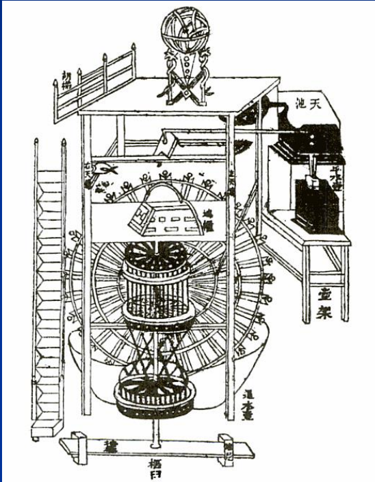
Fig. 631. General diagram of the works ( Hsin I Hsiang Fa Yao , ch. 3, p. 4a). On the right, the upper reservoir tank ( thien chhih ) with the constant-level tank ( ping shui hu ) beneath it. In the centre, foreground, the 'earth horizon' box ( ti kuei ) in which the celestial globe is mounted; below, the time-keeping shaft and wheels supported in the mortar-shaped end-bearing ( shu chiu ). Behind, the main driving wheel with its spokes and scoops; above, the left and right upper locks ( tsu yu thien so ) with the upper balancing lever and upper link, curiously drawn, still higher.
