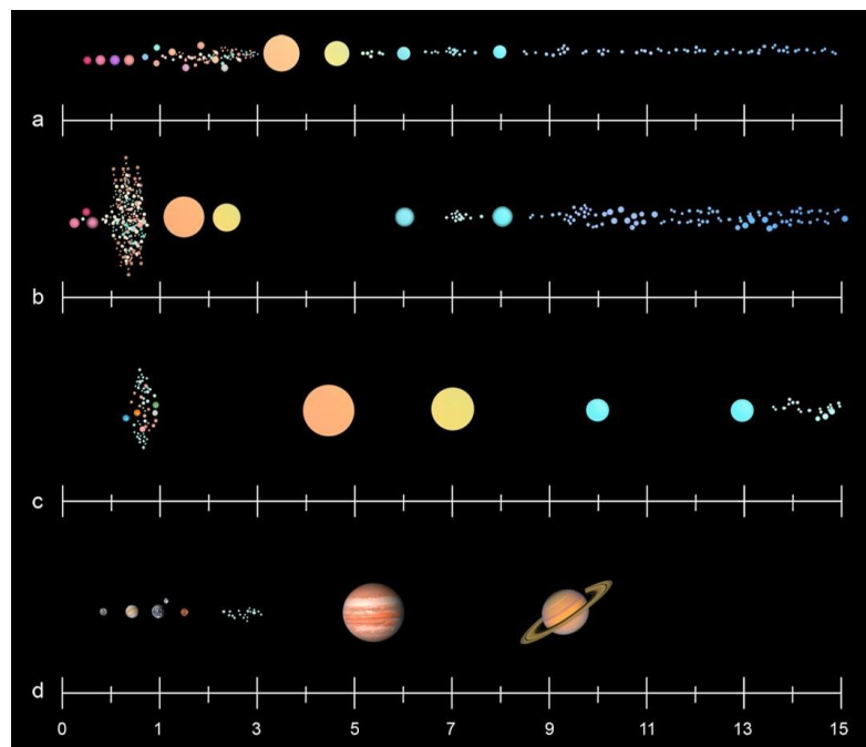
Fig. 7: Schematic representation of the “grand tack” hypothesis to explain the formation of our solar system and its planets; a) beginning of the model with the formation of the giant planets in progress, then b) first migration of Jupiter towards the sun with Saturn, c) second migration of Jupiter towards the outer solar system carrying Saturn and pushing asteroids and comets beyond 13 AU, d) position of the planets currently with the asteroid belt between 2 and 3 AU. @ Black Alley
