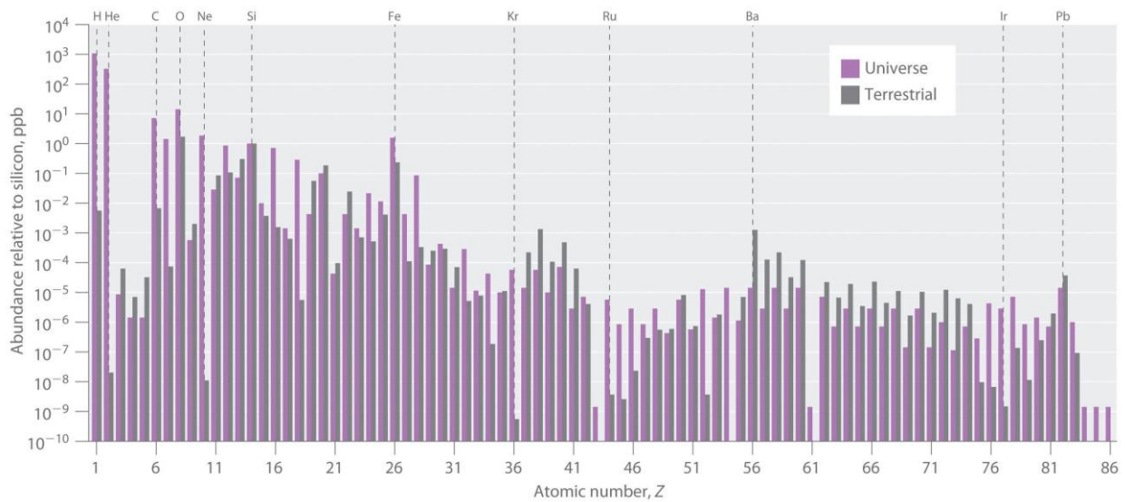
Fig. 5: Abundance of chemical elements in the Earth and Universe (logarithmic scale). The most abundant elements after hydrogen and helium are oxygen, carbon, and nitrogen, apart from the inert gas, neon and closely followed by iron and nickel.
