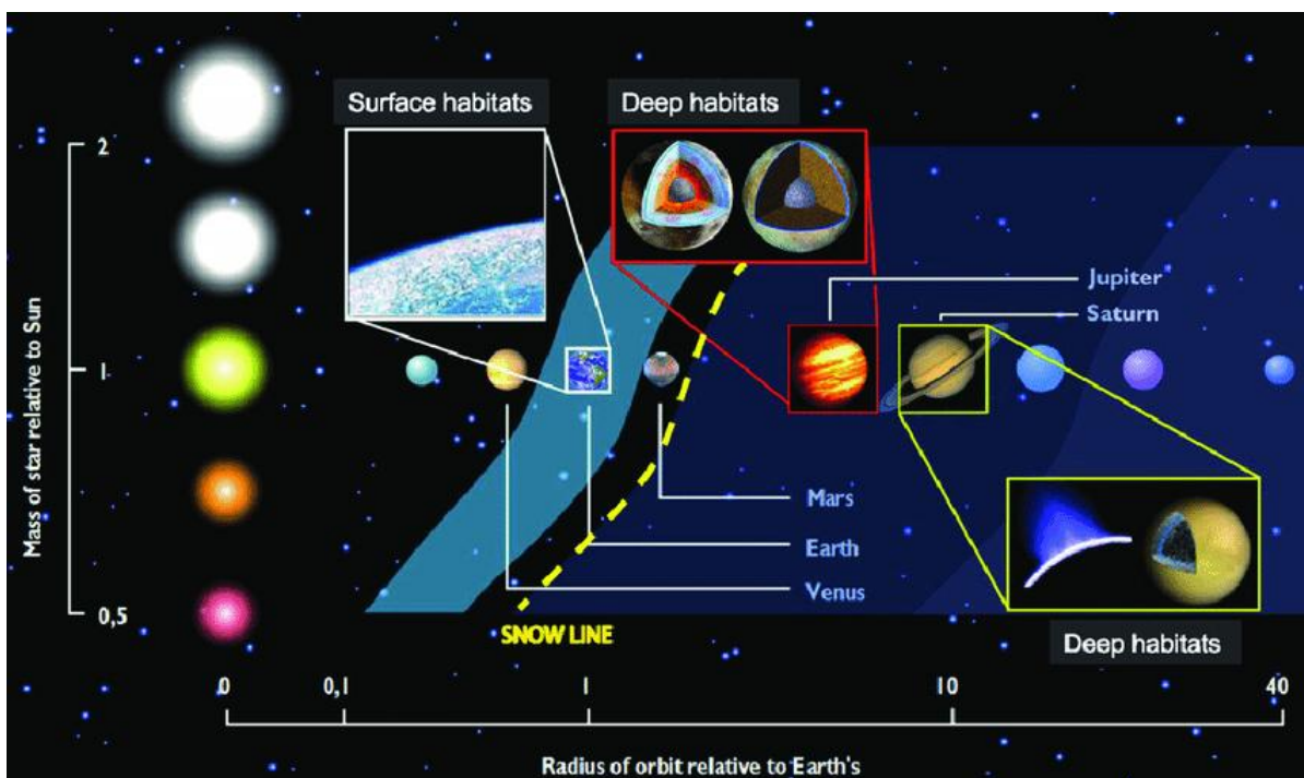
Fig. 6: Schematic representation of habitable zones in the solar system. The habitable zone is defined where there is liquid water: this zone depends on the mass of the star and the distance of the body from the star for the water to be stable on the surface or under it. With this definition and in our solar system, the Earth would be just in the middle of the habitable zone while Mars is at the limit. The icy satellites of Jupiter and Saturn would also be habitable bodies due to the presence of liquid water under their layer of ice (Credits: Neal Powell, Imperial College, London).
