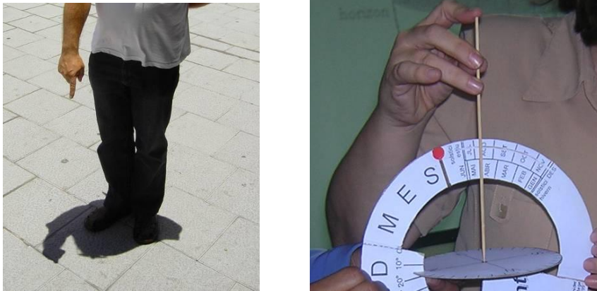
Fig. 26a: Small shadow (the Sun is almost at the zenith in a place near the equator). Fig. 26b: Simulating the Sun at the Zenith in Honduras (latitude 15° N).
