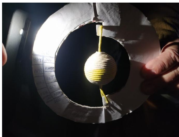
Fig. 31: Summer in the Northern Hemisphere and Winter in the Southern Hemisphere.
