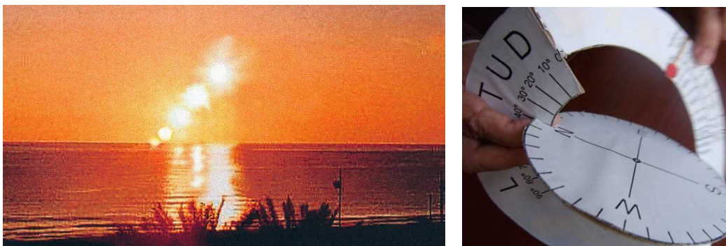
Fig. 17a and 17b: Sun rising in Gandia (Spain) 41^\circ\text{N} . The angle of the Sun's path relative to the horizon is 90 minus the latitude (Photo: Rosa M. Ros, Spain).
