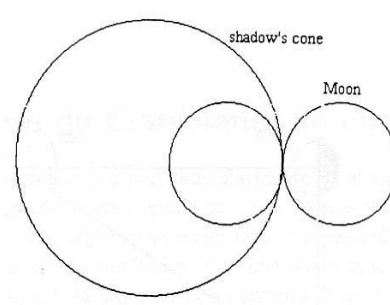
Fig.16b: Measuring the diameter of the Moon.
