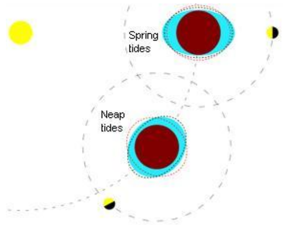
Fig. 22: Spring tides and neap tides.
