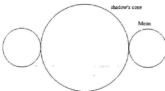
Fig. 16a: Measuring the cone of shadow.
