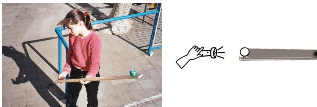
Fig.5a and 5b: Lunar eclipse simulation.
